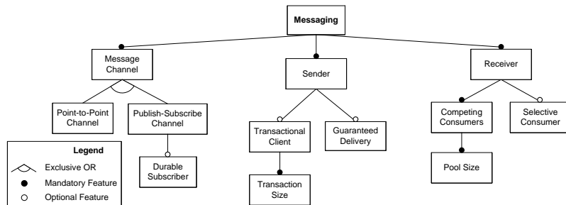
Fig. 3. MOM Adaptor Feature Model.
