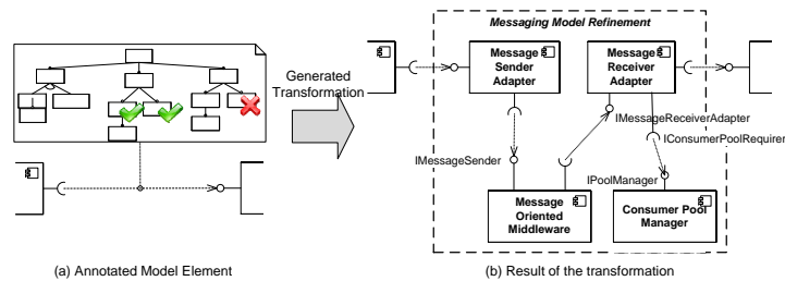
Fig. 5. Transformation integrating MOM Adaptor.
