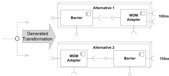
Fig. 7. Completion Alternatives.
