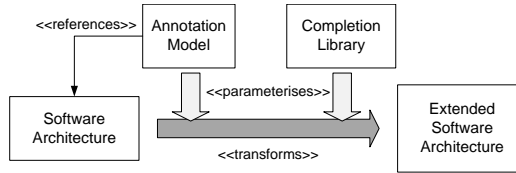
Fig. 4. Transformation integrating performance completions.
