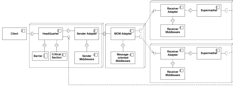
Fig. 8. Resulting Architecture.
