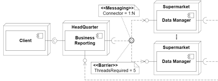
Fig. 6. Annotated Architecture.
