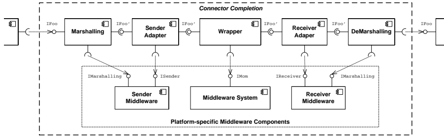
Fig. 12. Connector Middleware Completion.
